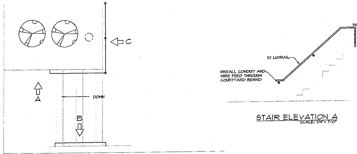
ILLUMINATED HANDRAIL PLAN SCALE: 1/4" = 1'-0"
