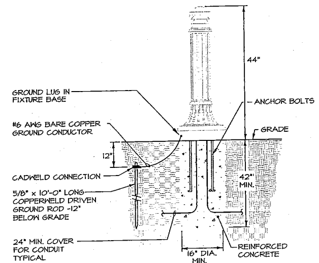
TYPE 'SC' BOLLARD FIXTURE DETAIL NO SCALE
